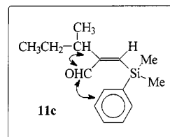
Figure 1. Determination of the configuration of 2-(dimethylphenylsilylmethylene)-3-methylpentanal ( 11c ) by NOE experiments.
